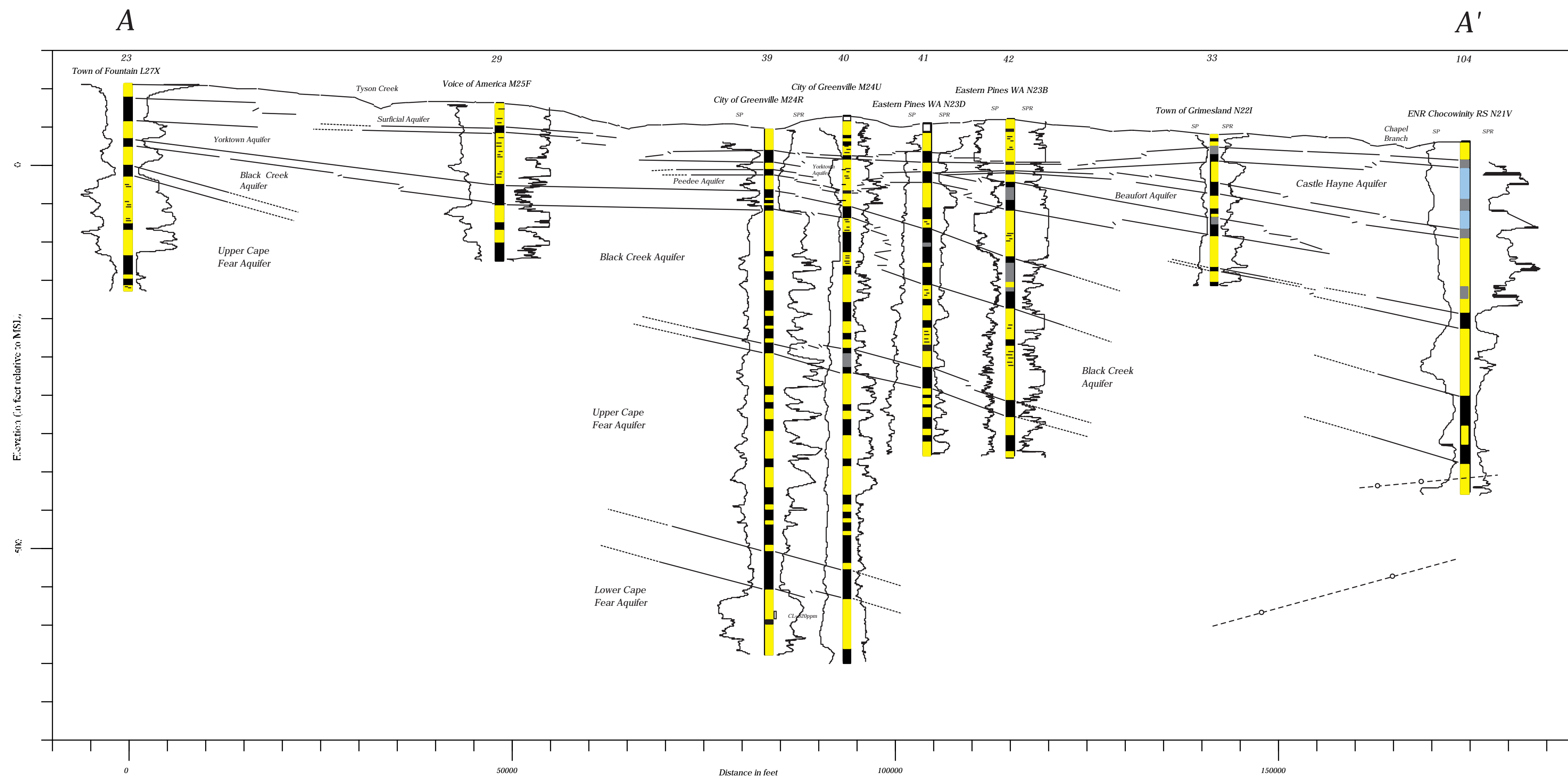
Plate 2: Northwest to Southeast Hydrogeologic Cross Section A-A' through Wilson, Pitt and Beaufort Counties, NC
