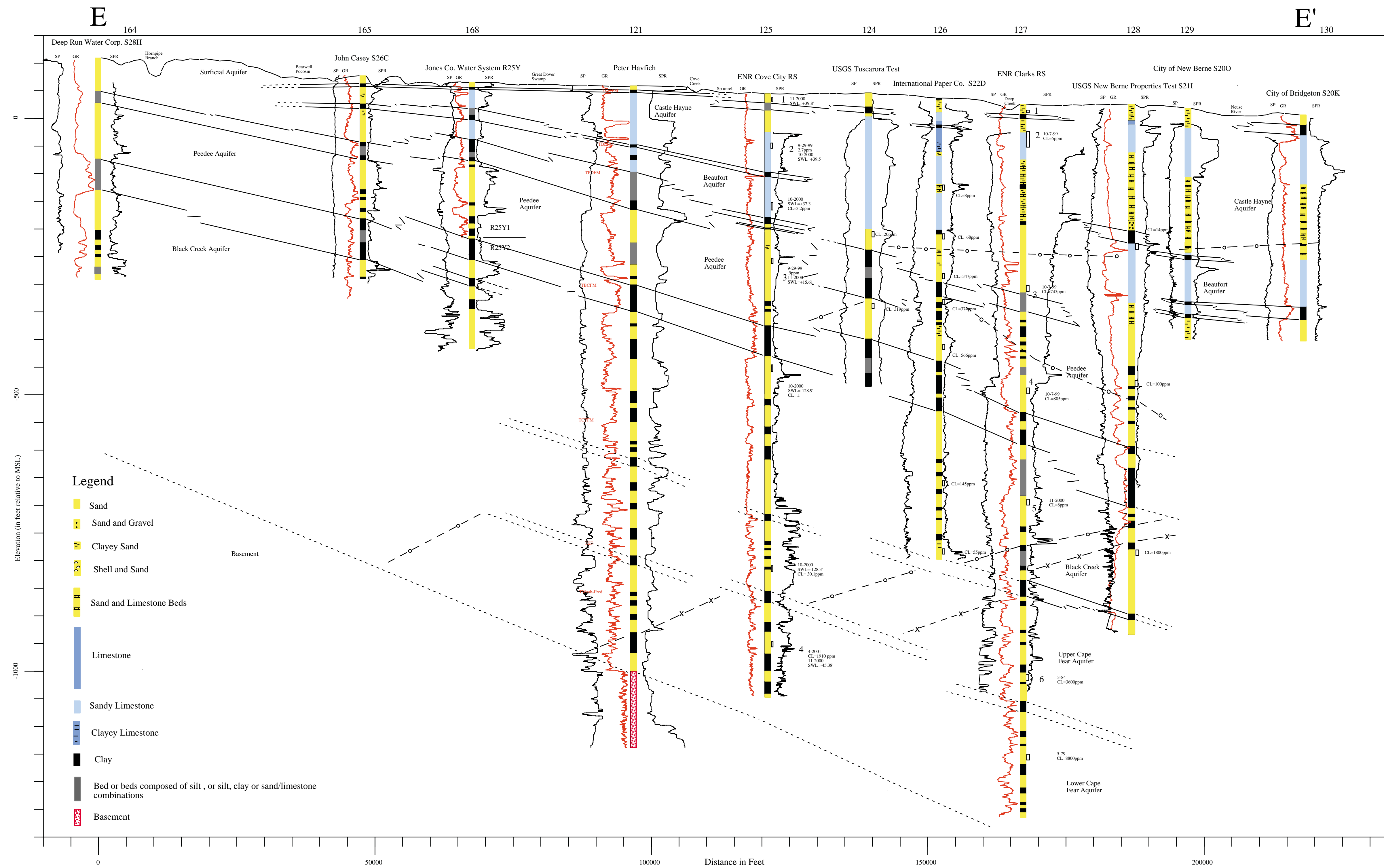
Plate 6: West to East Hydrogeologic Cross Section E-E' through Lenoir, Jones, and Craven Counties, NC
