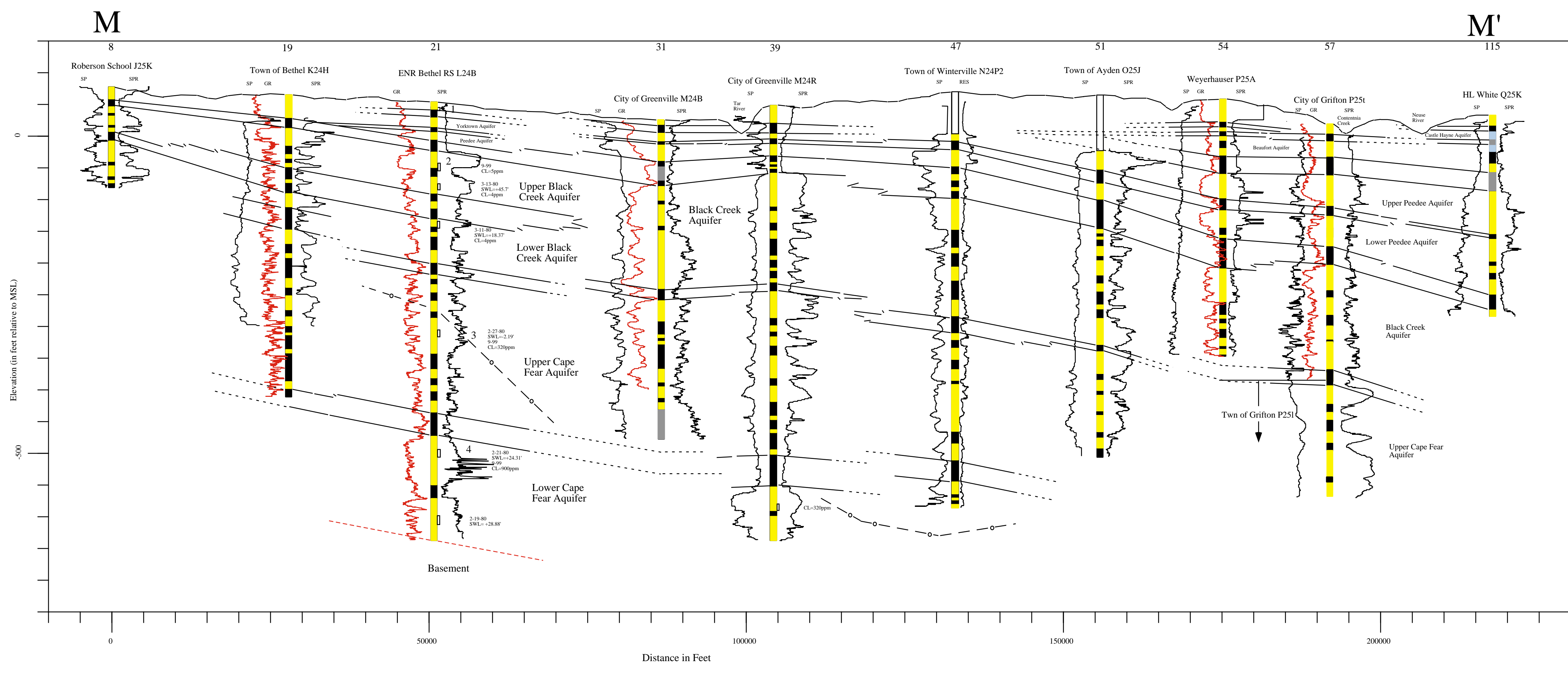
Plate 15: North to South Hydrogeologic Cross Section M-M' through Edgecombe, Pitt, and Craven, Counties, NC
