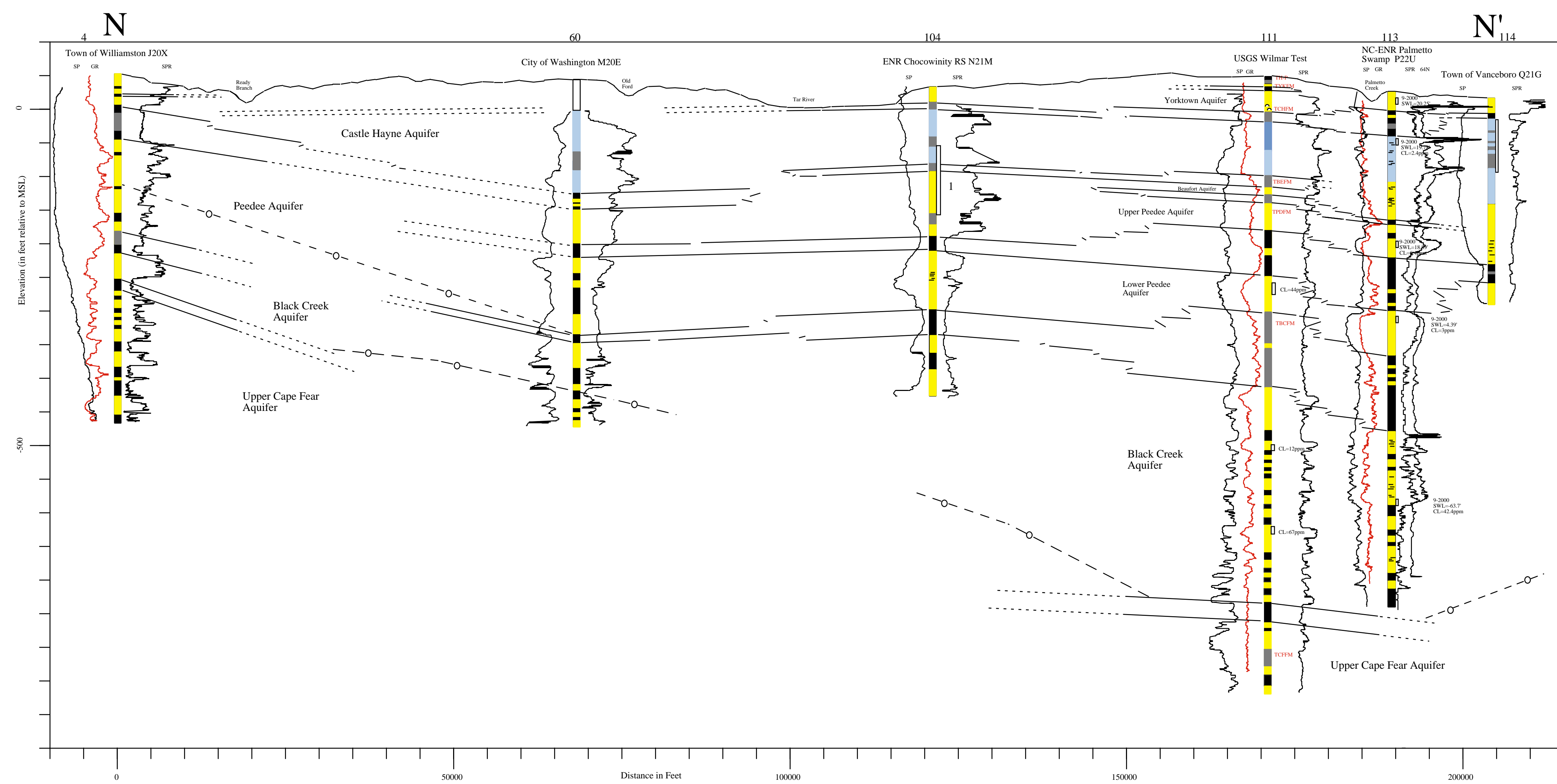
Plate 17: North to South Hydrogeologic Cross Section N-N' through Martin, Beaufort, and Craven Counties, NC
