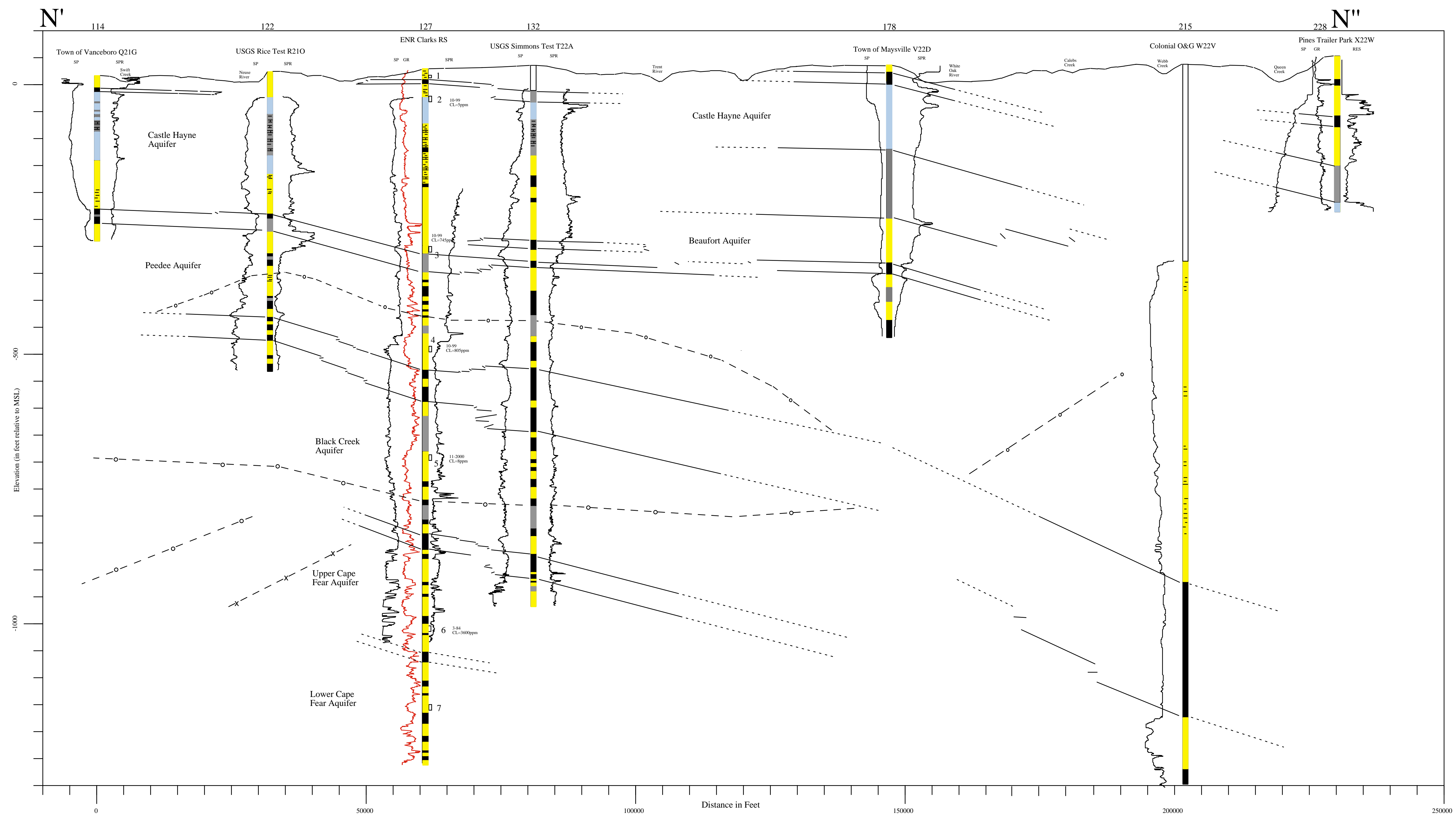
Plate 18: North to South Hydrogeologic Cross Section N'-N'' through Craven, Jones, and Onslow Counties, NC
