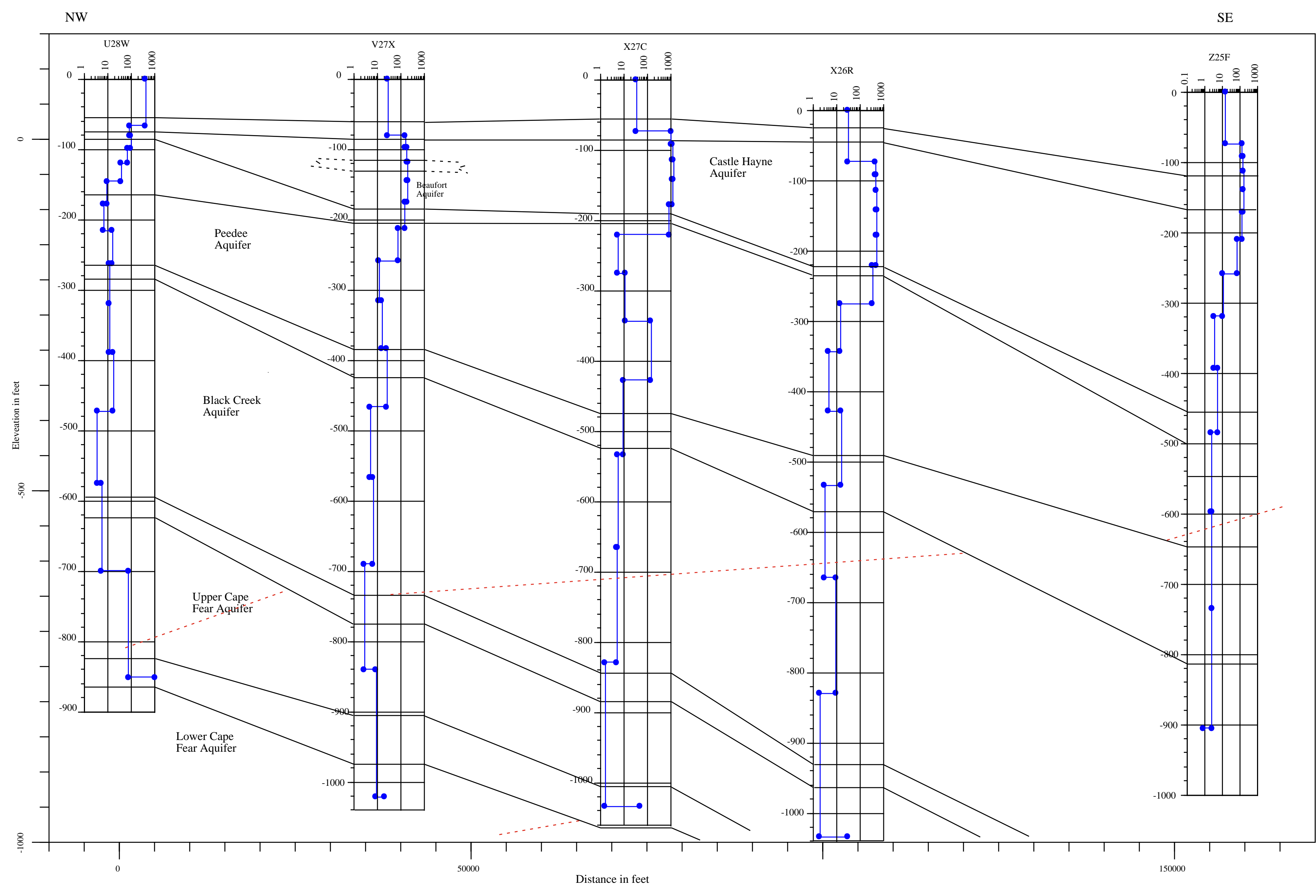
Plate 20: Cross Section TDEM a-a' through Duplin and Onslow Counties, NC Hydrogeologic Unit Correlation Lines are Derived From Elevation Contours From Hydrogeologic Unit Elevation Maps and are not based on TDEM response. Correlation Line TDEM Apparent Resistivity Approximate Freshwater/Saltwater Interface
