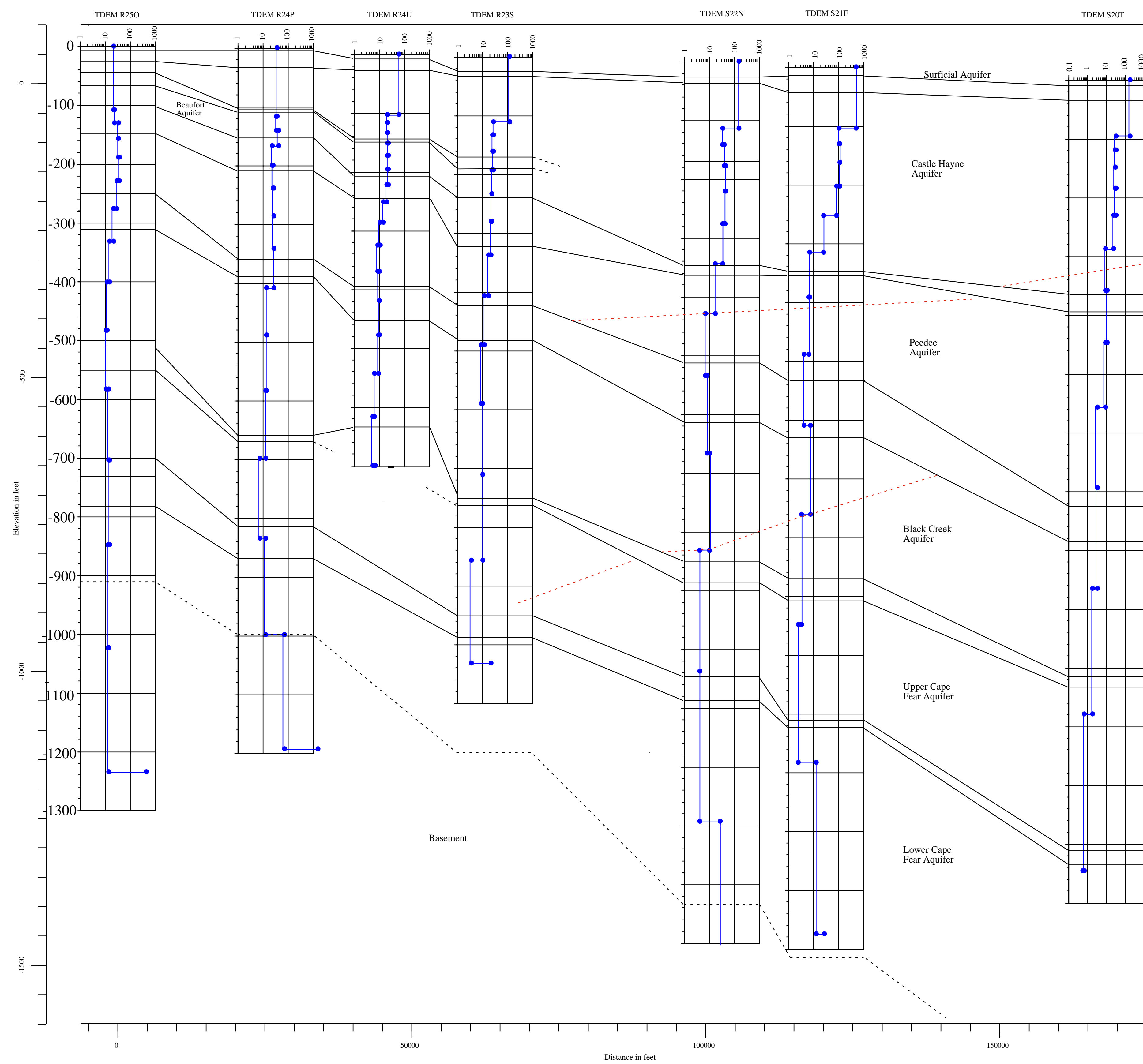
Plate 21: Cross Section TDEM b-b' through Jones and Craven Counties, NC Hydrogeologic Unit Correlation Lines are Derived From Elevation Contours From Hydrogeologic Unit Elevation Maps and are not based on TDEM response.
