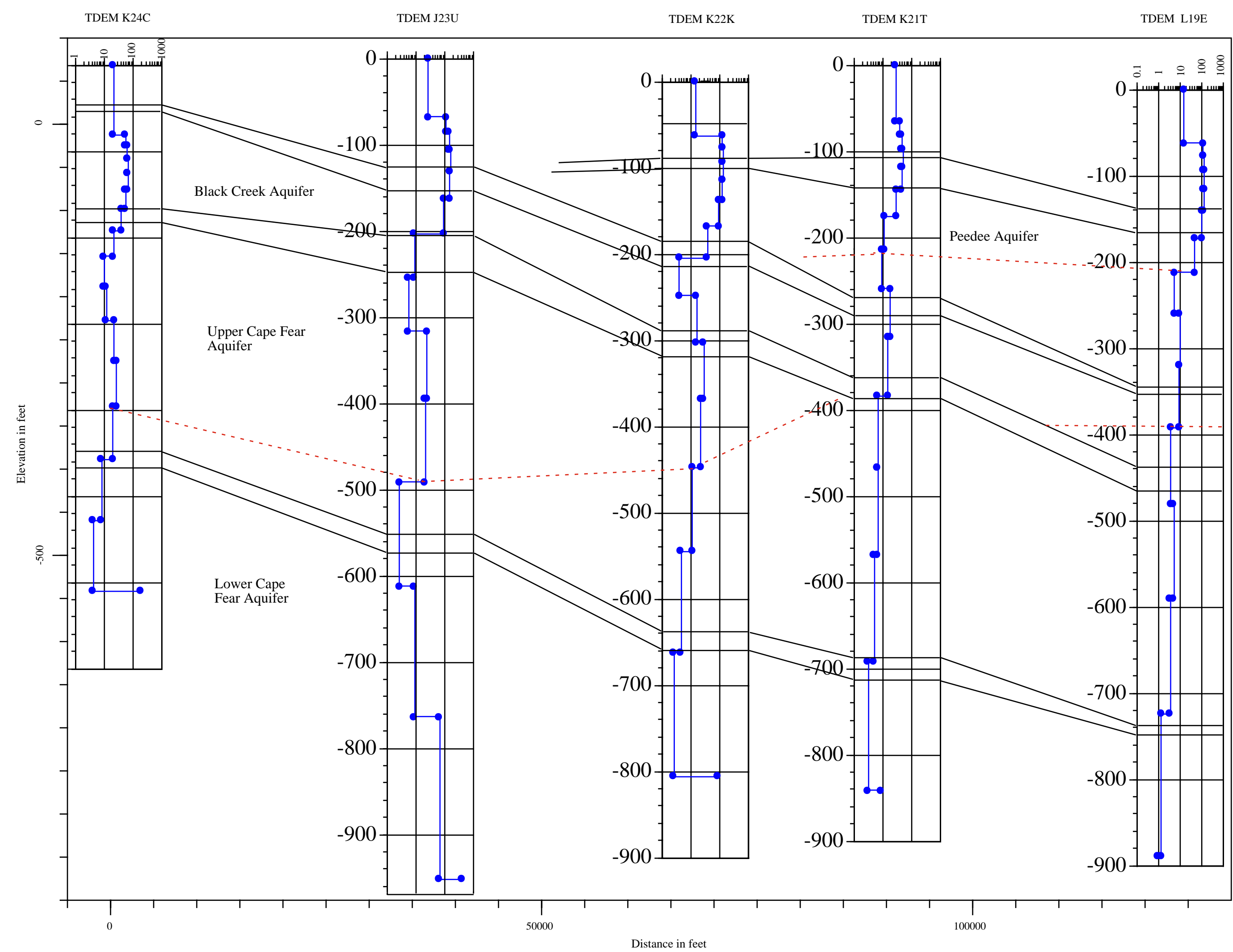
Plate 23: Cross Section TDEM d-d' through Edgecombe and Martin Counties, NC Hydrogeologic Unit Correlation Lines are Derived From Elevation Contours From Hydrogeologic Unit Elevation Maps and are not based on TDEM response. Correlation Line TDEM Apparent Resistivity Approximate Freshwater/Saltwater Interface
