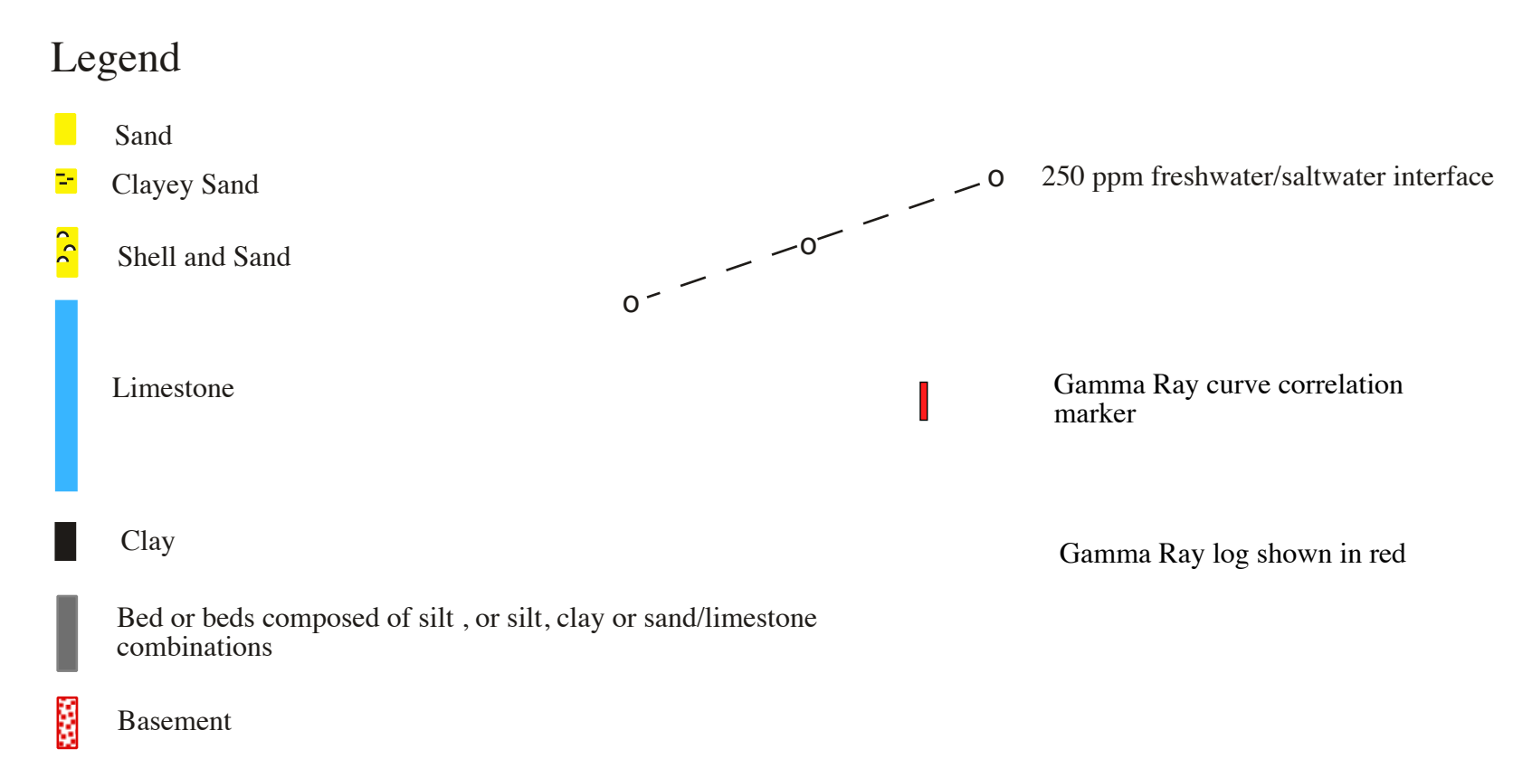
Plate 2. West to East Hydrogeologic Cross Section A-A' through Washington, Tyrrell and Dare Counties, NC
