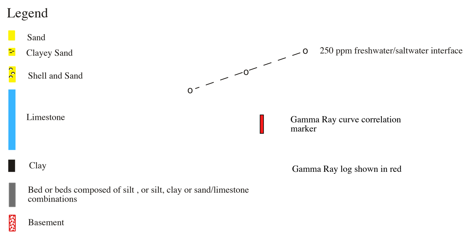
Plate 4. West to East Hydrogeologic Cross Section C-C' through Beaufort, Hyde and Dare Counties, NC
