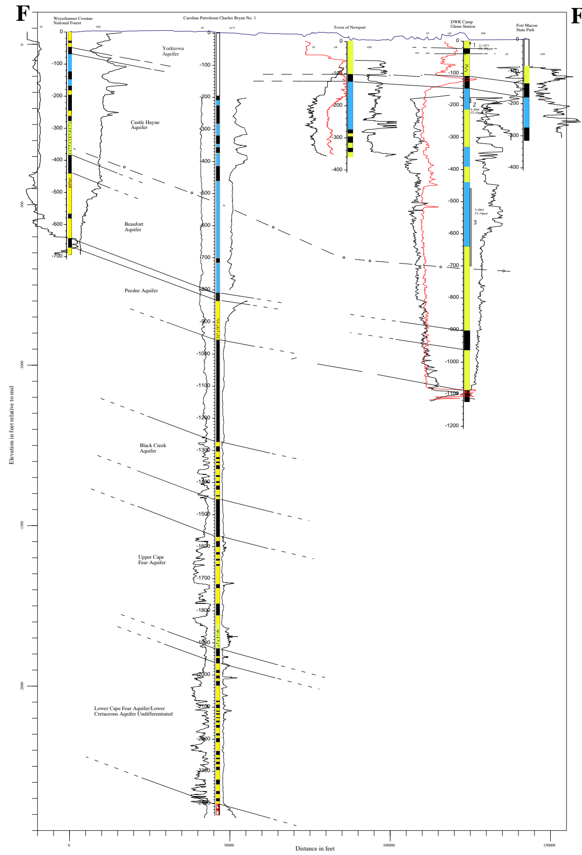
Plate 7. Northwest to Southeast Hydrogeologic Cross Section F-F' through Craven and Cartaret Counties, NC
