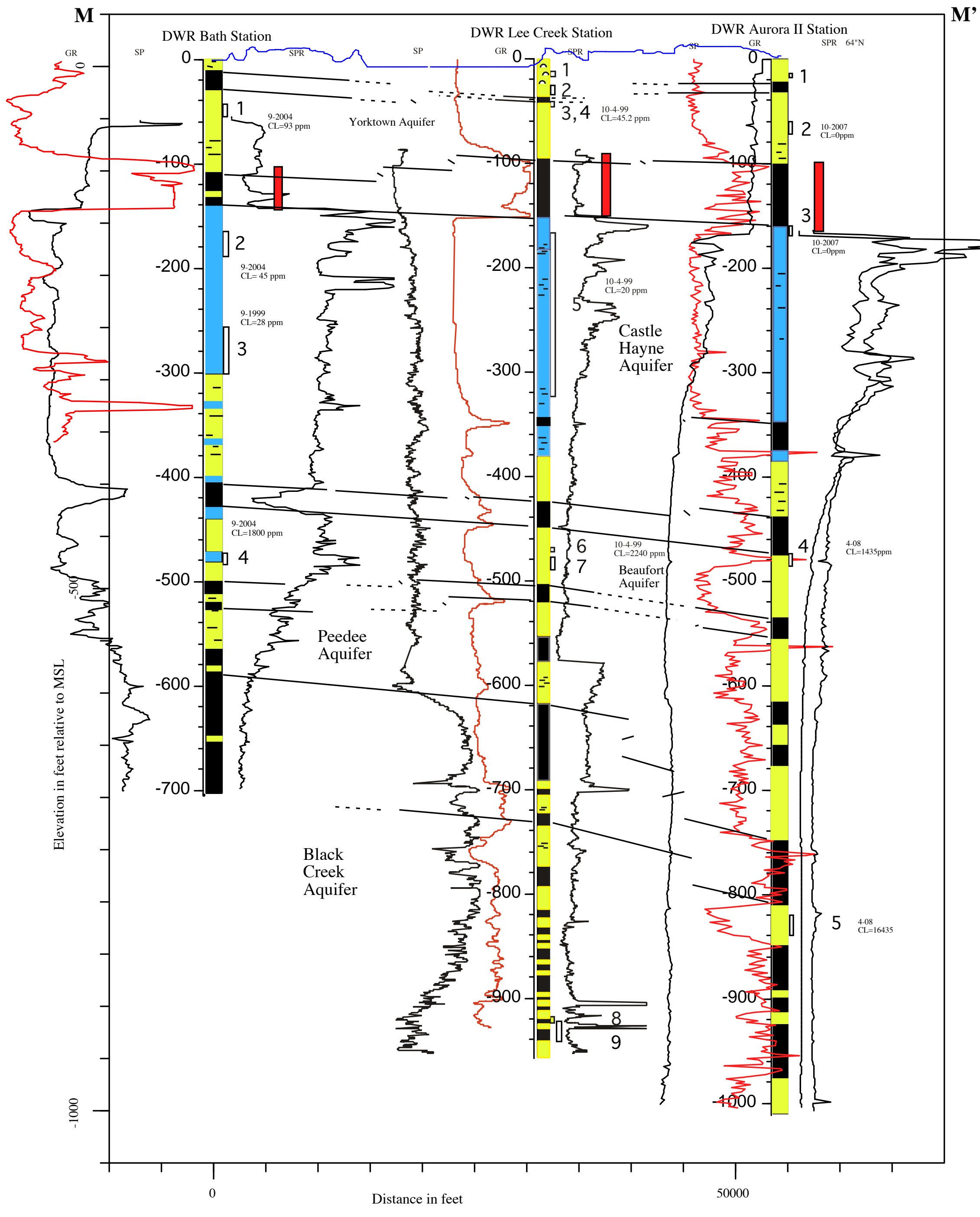
Plate 14: Hydrogeologic Cross Section M-M' through Beaufort County, NC
