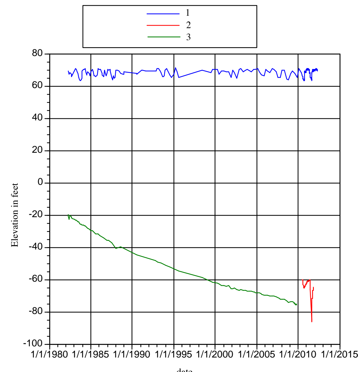
Hydrograph: DWR Roxobel Monitoring Station, Bertie County
