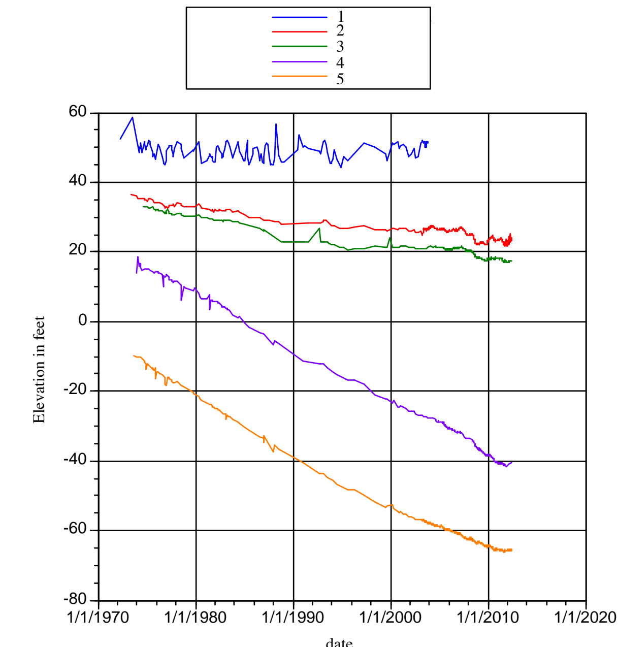
Hydrograph: DWR Cremo Monitoring Station, Bertie County
