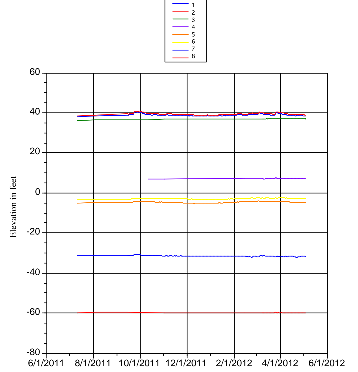
Hydrograph: DWR Windsor Monitoring Station, Bertie County
