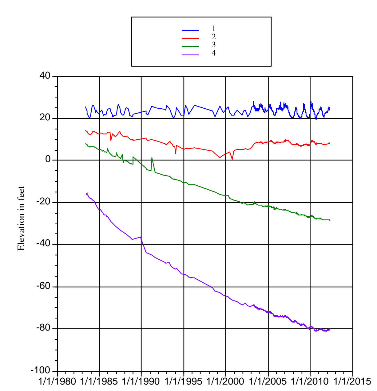
Hydrograph: DWR Lewiston Monitoring Station, Bertie County
