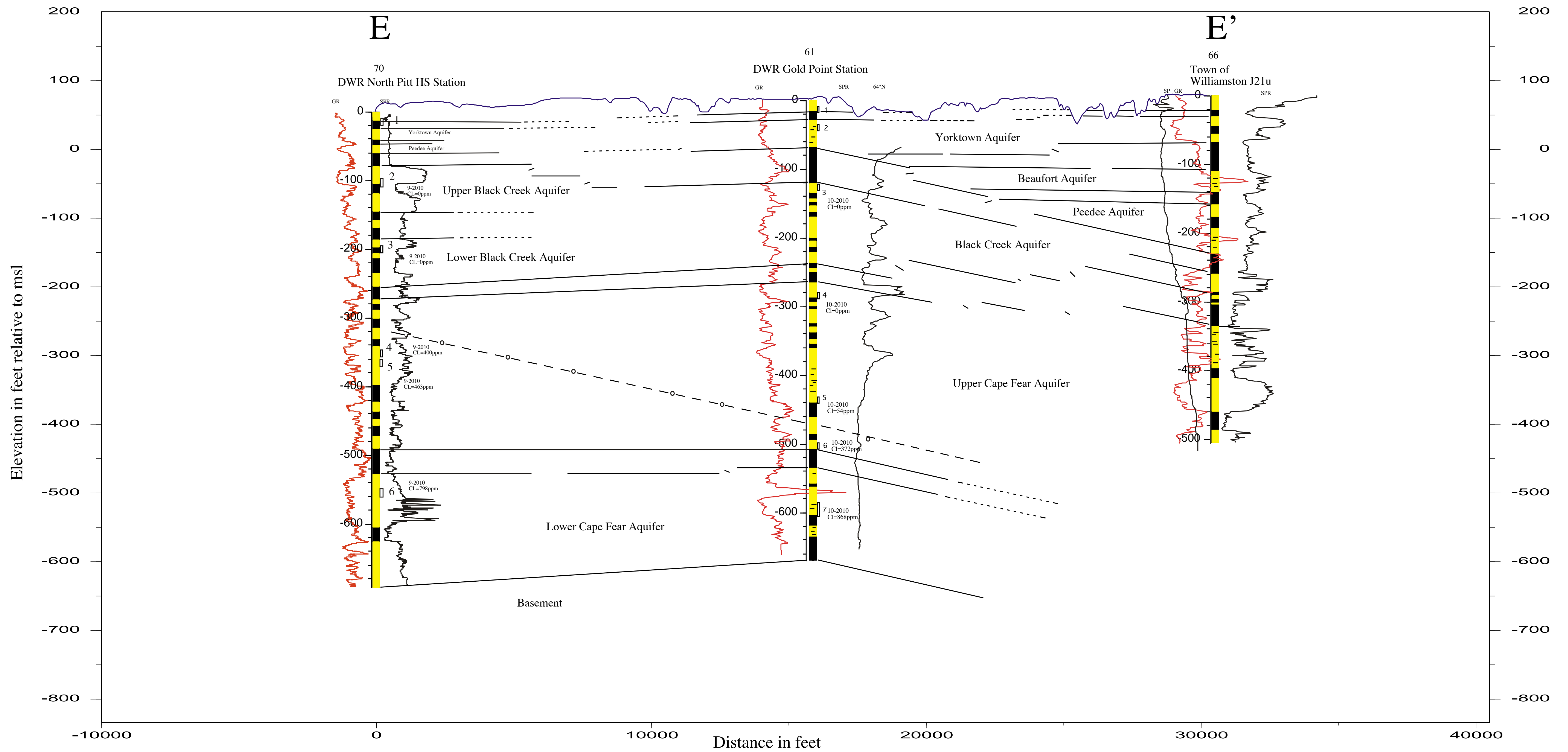
Plate 6. Southwest to Northeast Hydrogeologic Cross Section E-E' through Pitt and Martin Counties, NC
