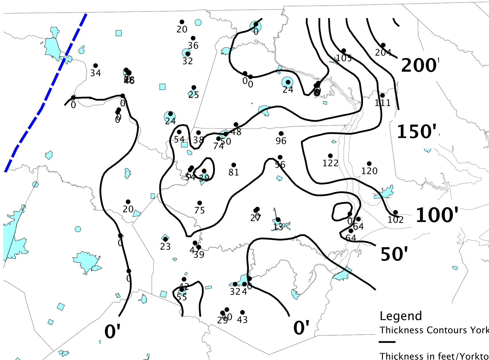
Plate 15 Thickness Contours: Yorktown Aquifer in the NC Northwestern Coastal Plain
