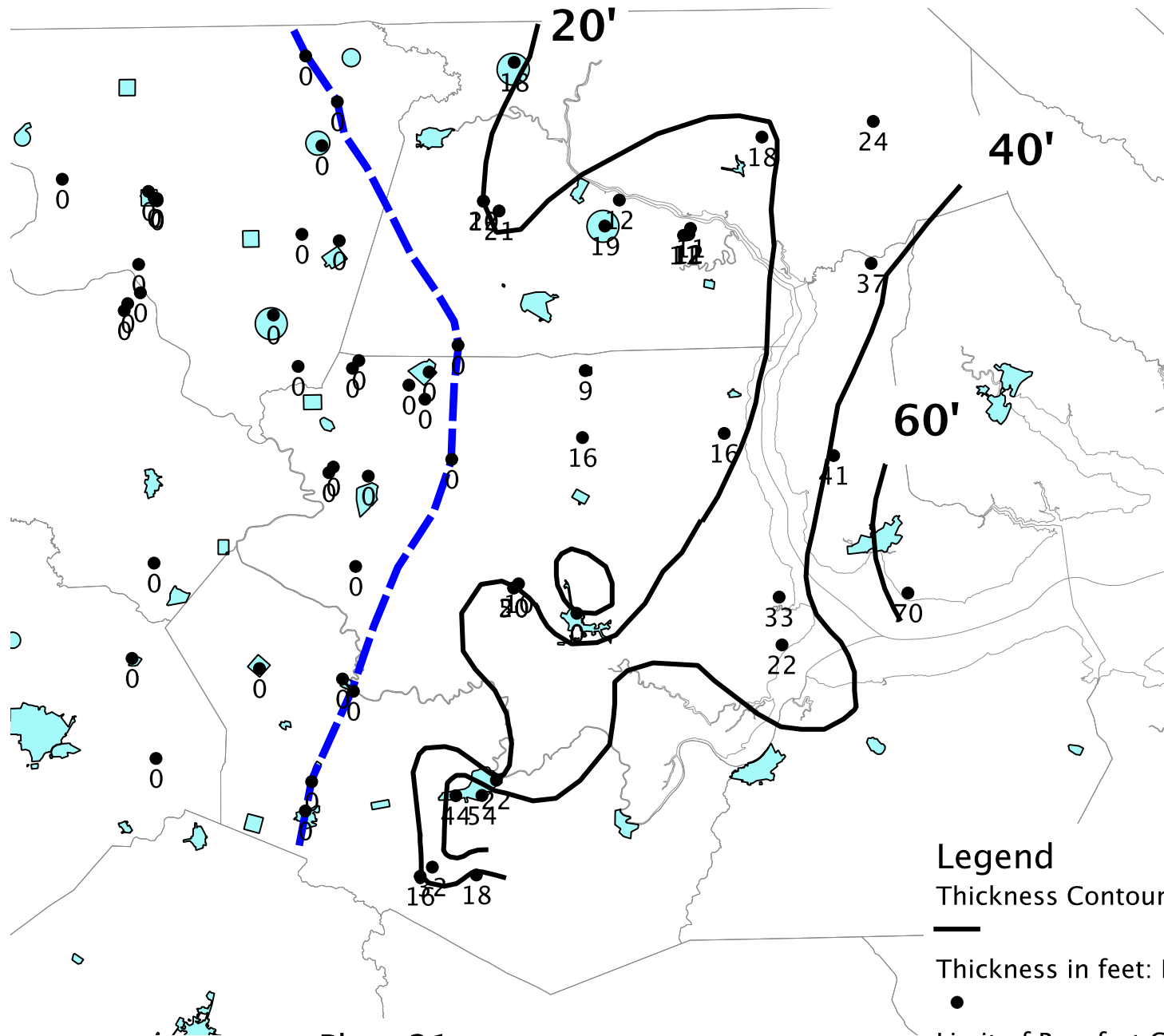
Plate 21 Thickness Contours: Beaufort Confining Unit in the NC Northwestern Coastal Plain
