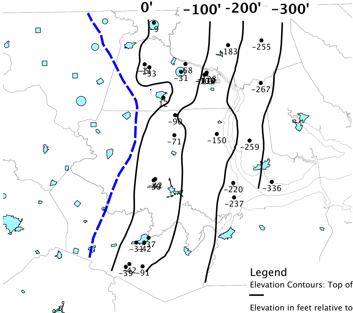
Plate 22 Elevation Contours: Top of the Beaufort Aquifer in the NC Northwestern Coastal Plain
