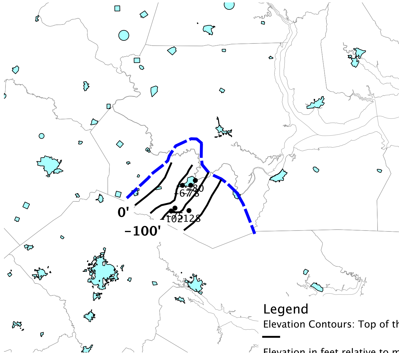
Plate 24 Elevation Contours: Top of the Peedee Confining Unit in the NC Northwestern Coastal Plain
