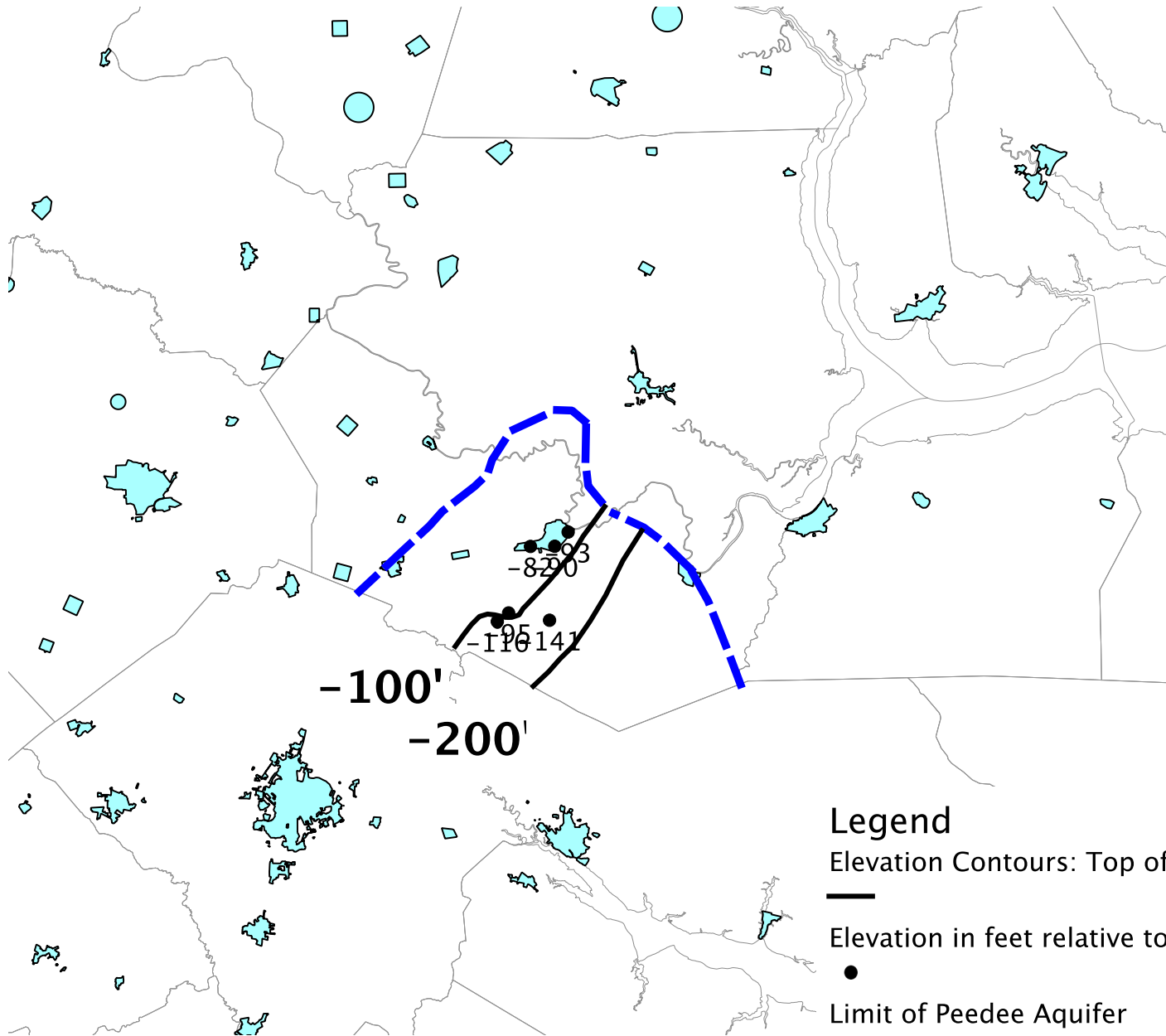
Plate 26 Elevation Contours: Top of the Peedee Aquifer in the NC Northwestern Coastal Plain
