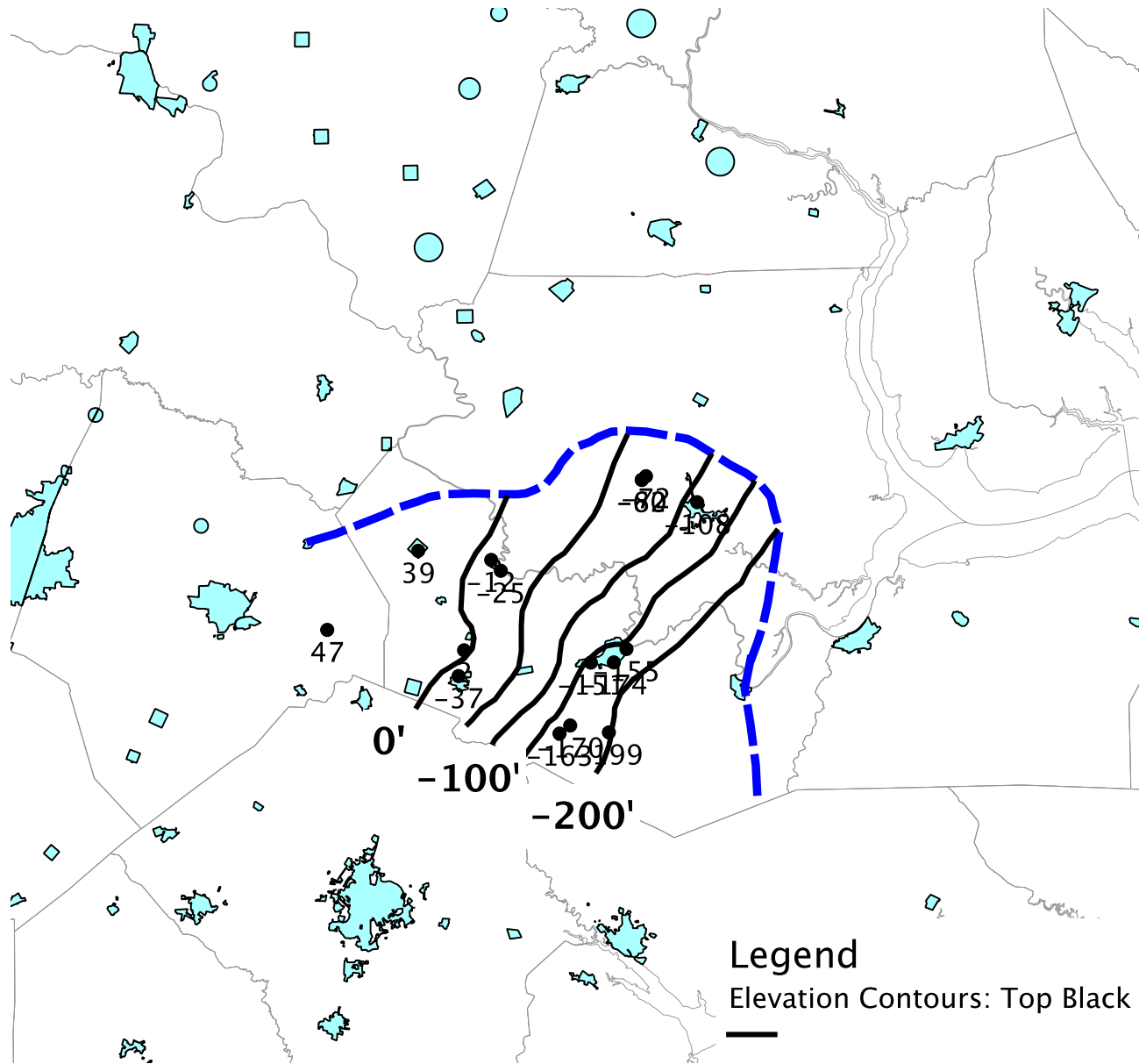
Plate 28 Elevation Contours: Top of Black Creek Confining Unit in the NC Northwestern Coastal Plain
