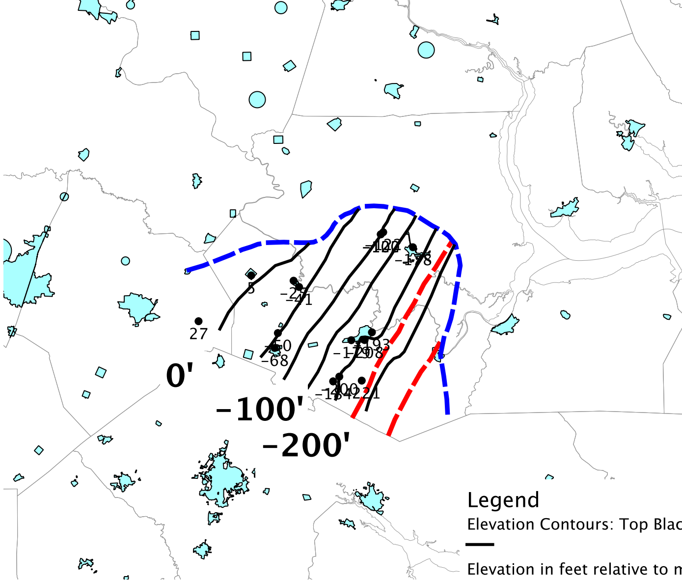
Plate 30 Elevation Contours: Top of Black Creek Aquifer in the NC Northwestern Coastal Plain
