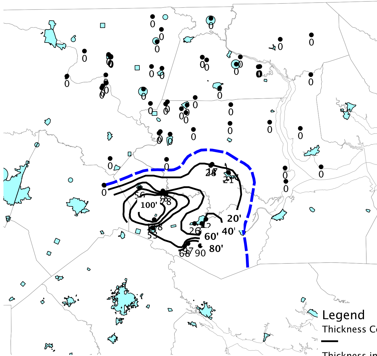
Plate 31 Thickness Contours: Black Creek Aquifer in the NC Northwestern Coastal Plain
