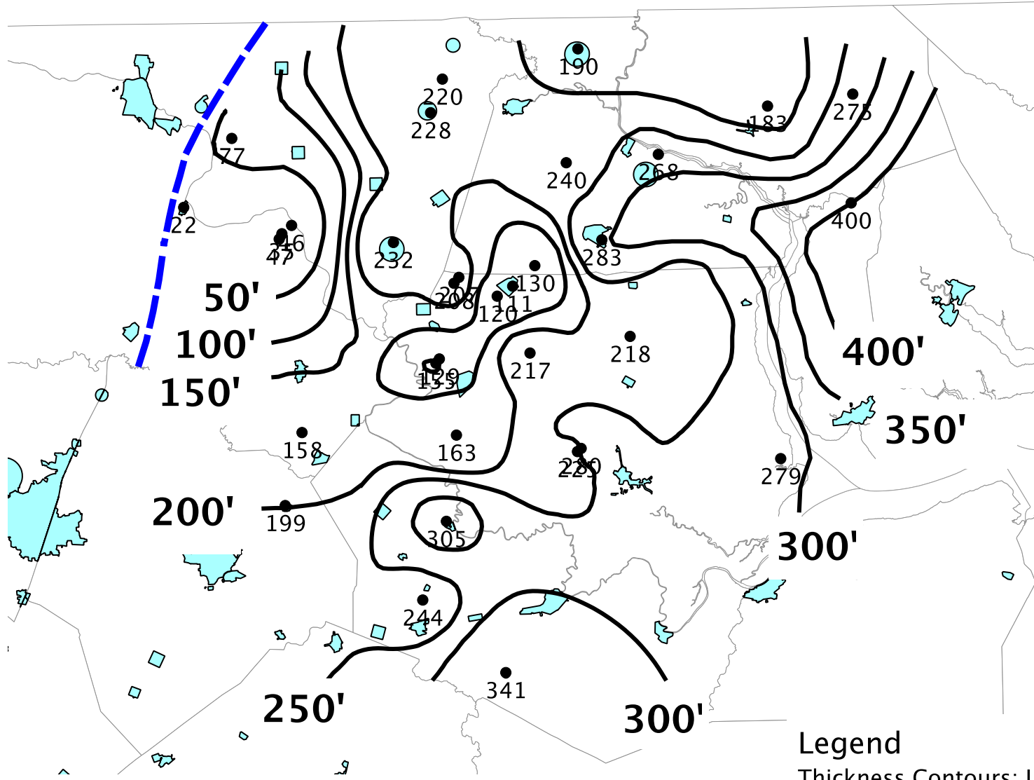
Plate 35 Thickness Contours: Upper Cape Fear Aquifer in the NC Northwestern Coastal Plain
