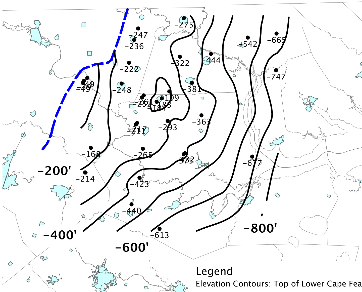
Plate 36 Elevation Contours: Top of the Lower Cape Fear Confining Unit in the NC Northwestern Coastal Plain
