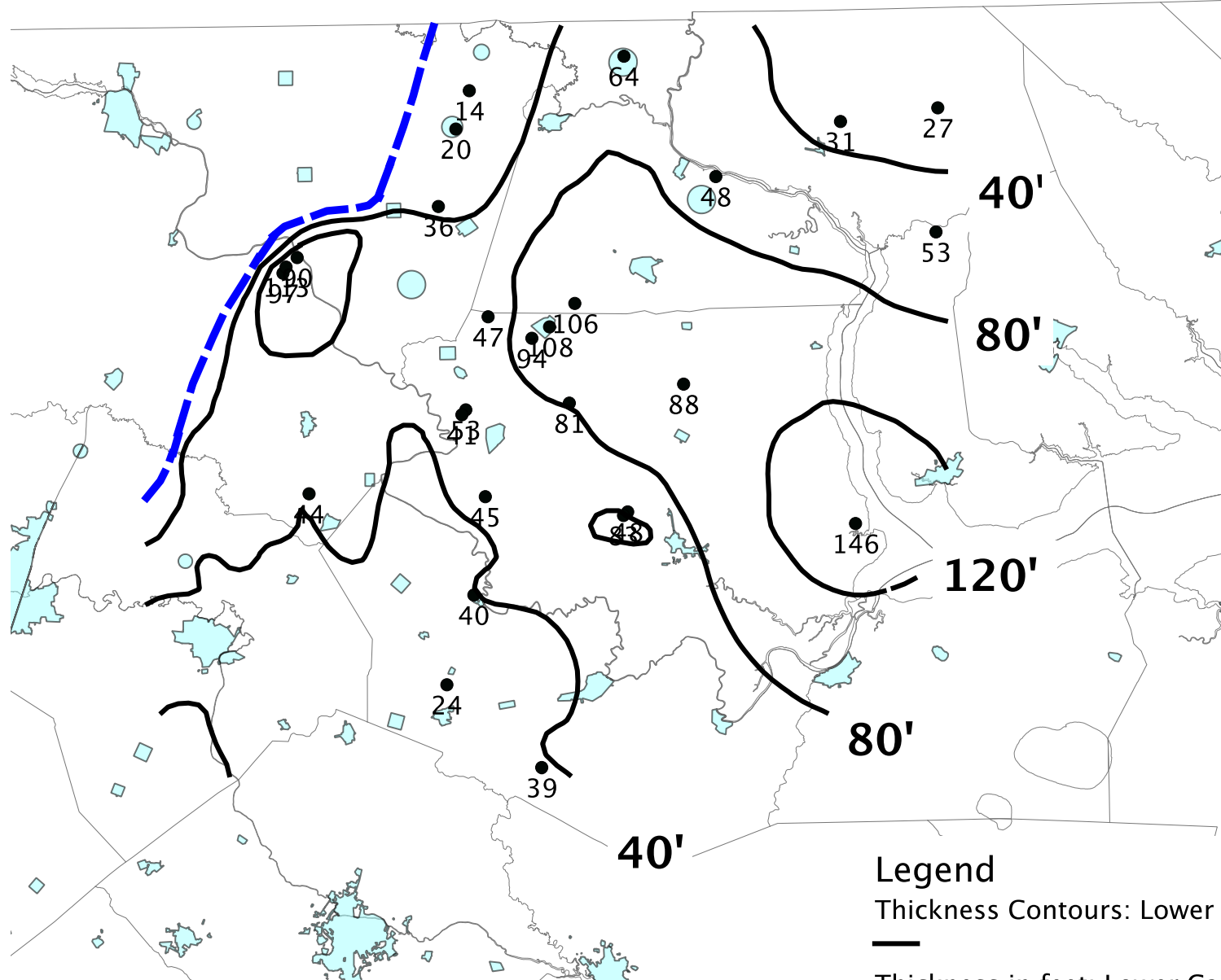
Plate 37 Thickness Contours: Lower Cape Fear Confining Unit in the NC Northwestern Coastal Plain
