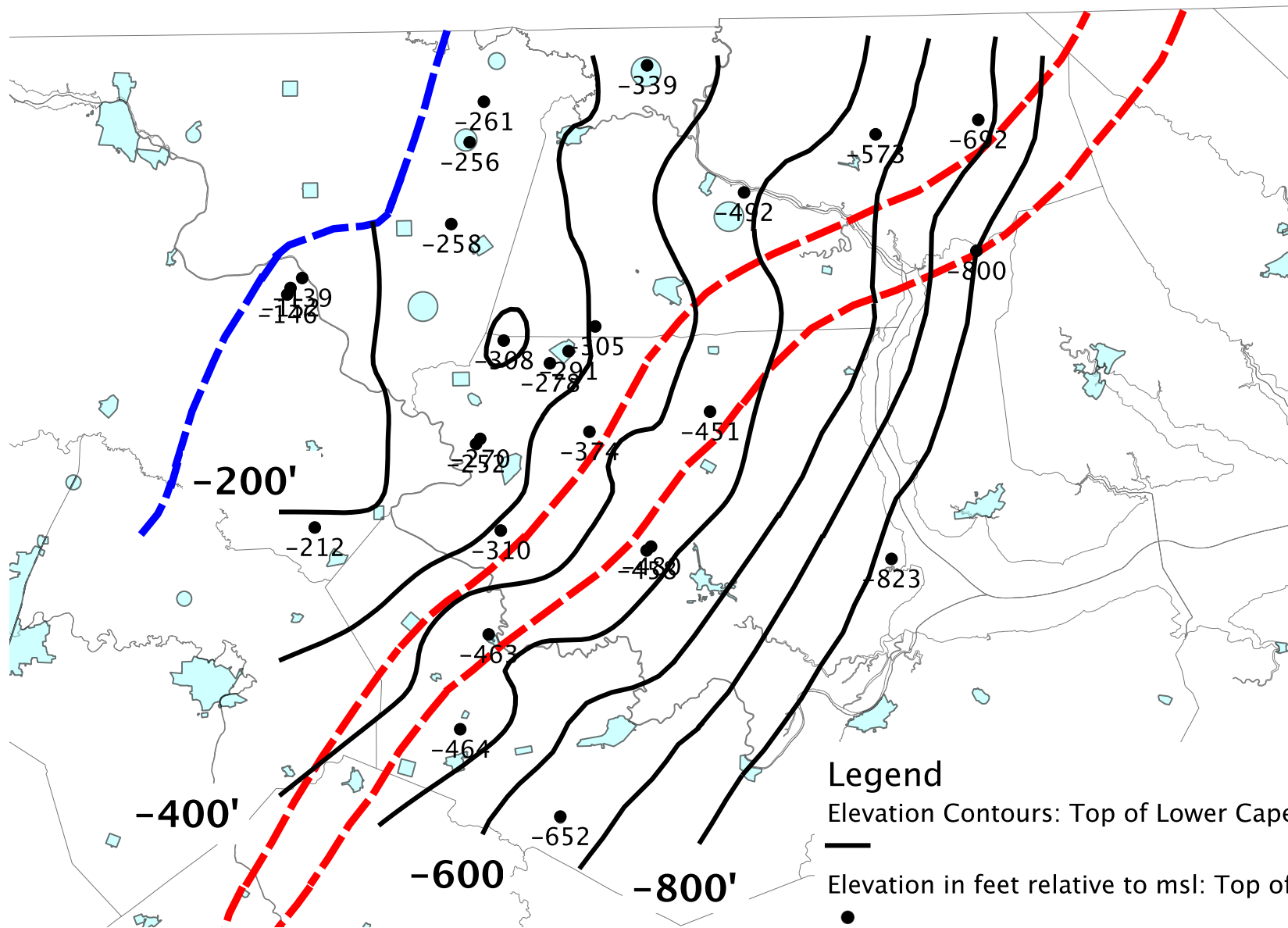
Plate 38 Elevation Contours: Top of the Lower Cape Fear Aquifer in the NC Northwestern Coastal Plain
