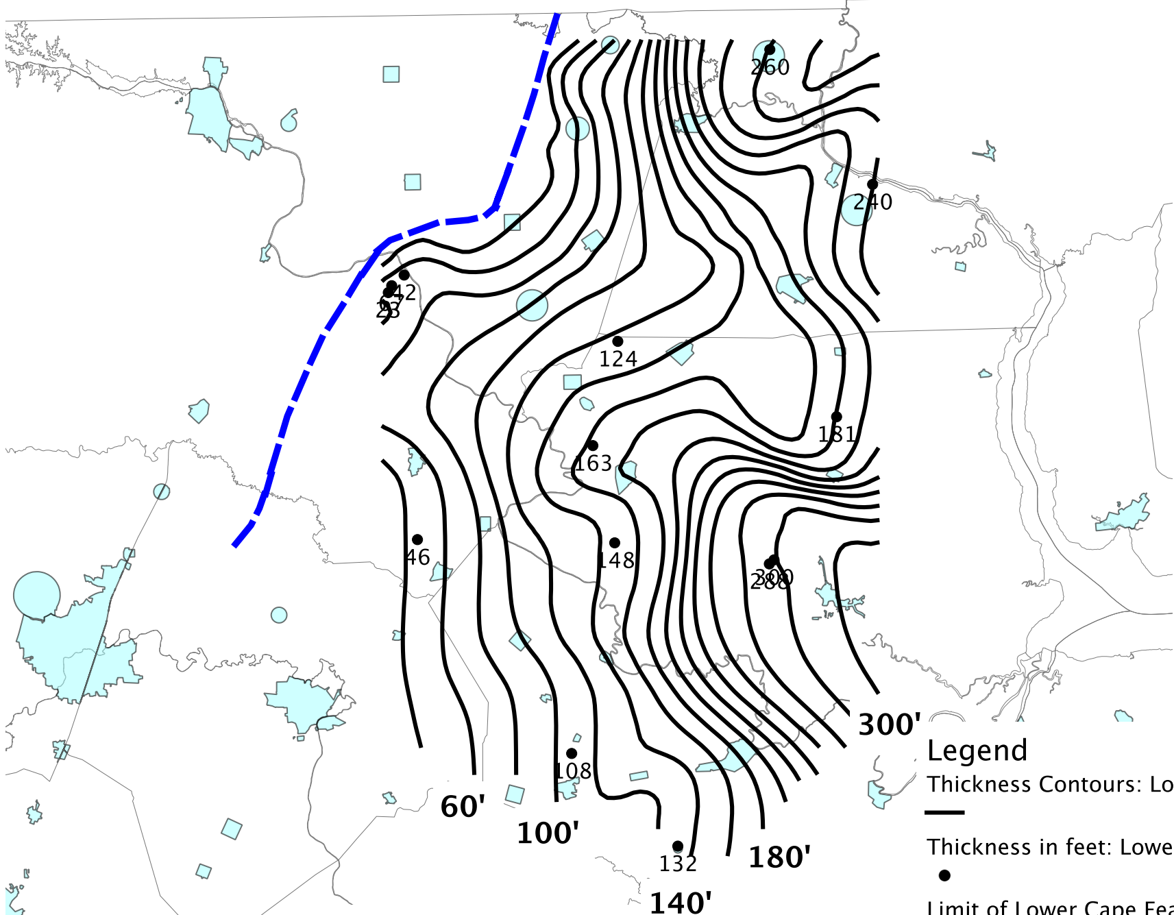
Plate 39 Thickness Contours: Lower Cape Fear Aquifer in the NC Northwestern Coastal Plain
