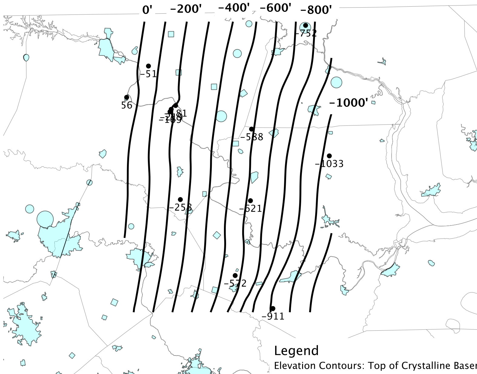
Plate 44 Elevation Contours: Top of Crystalline Basement Rock in the NC Northwestern Coastal Plain
