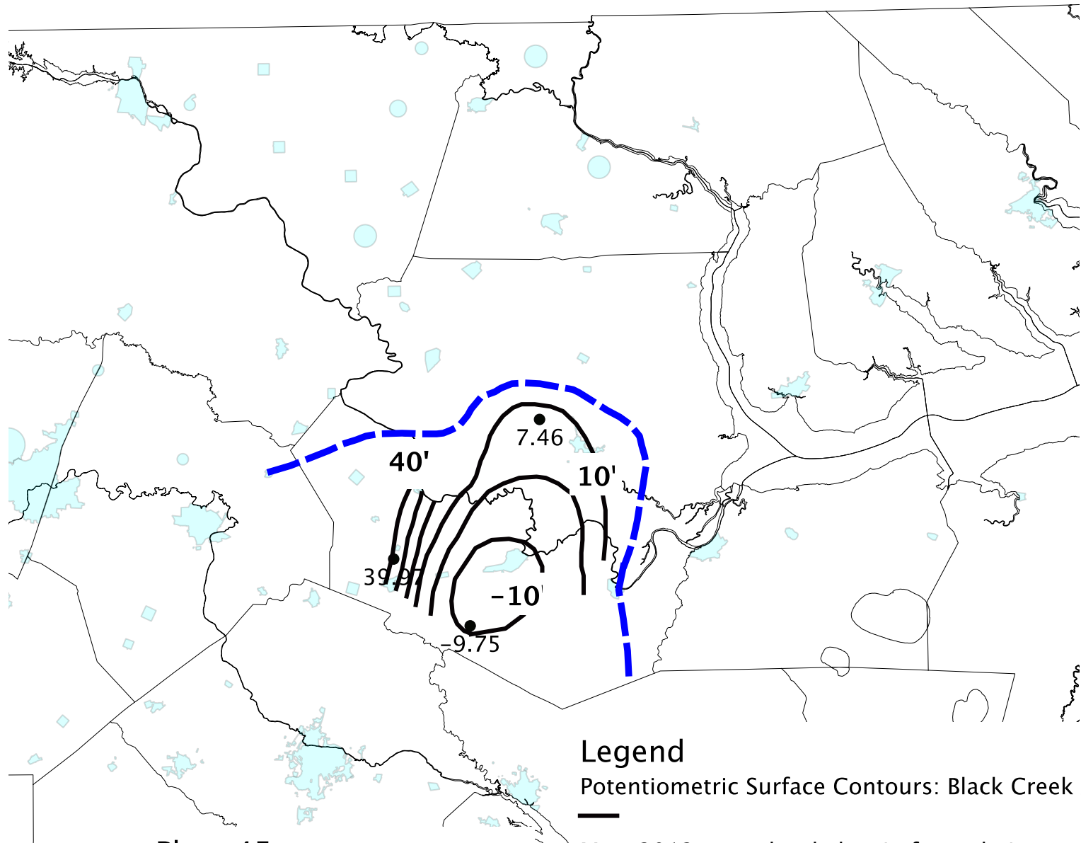
Plate 45 Potentiometric Surface Contours: Black Creek Aquifer in the NC Northwestern Coastal Plain
