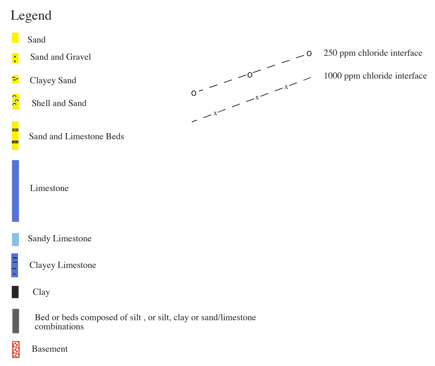
Plate 15. Southwest to Northeast Hydrogeologic Cross Section N-N' through Brunswick County, NC
