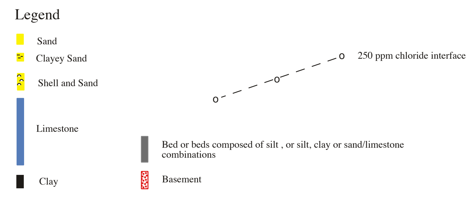
Plate 7: Northwest to Southeast Hydrogeologic Cross Section F-F' through Robeson, Bladen, and Columbus Counties, NC
