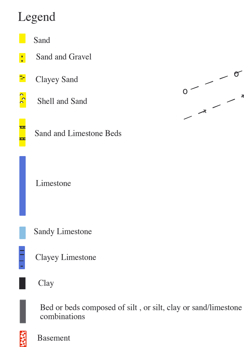
Plate 11. Northwest to Southeast Hydrogeologic Cross Section I-I' through Scotland, Robeson, Columbus and Brunswick Counties, NC
