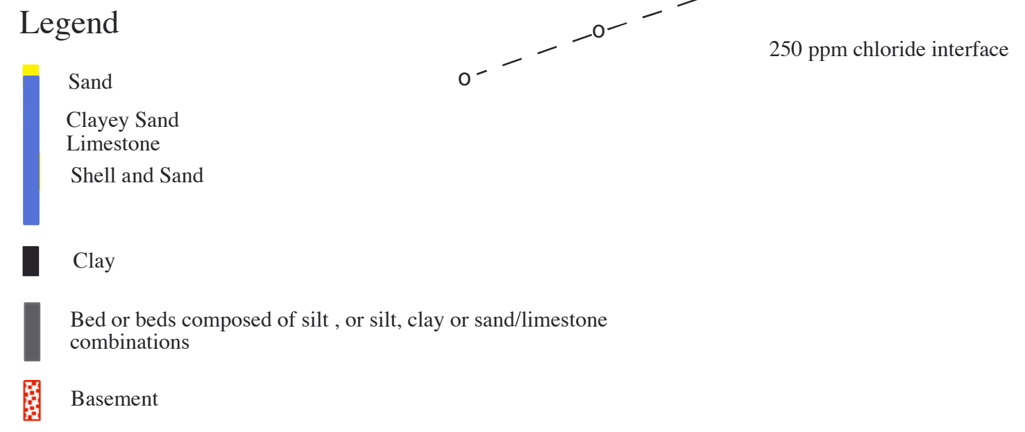
Plate 12. Southwest to Northeast Hydrogeologic Cross Section J-J' through Brunswick and Pender Counties, NC
