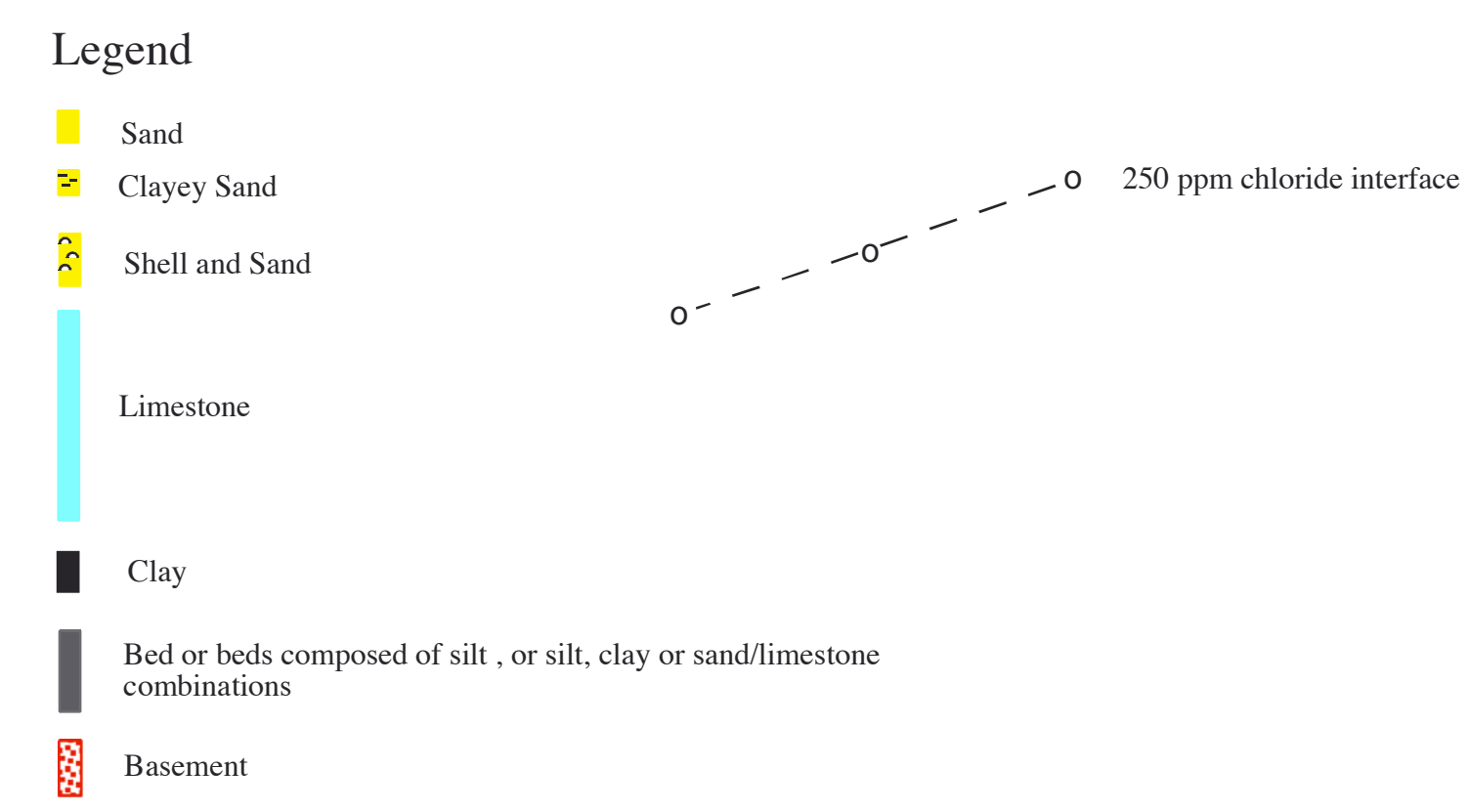
Plate 13. Northwest to Southeast Hydrogeologic Cross Section K-K' through Brunswick County, NC
