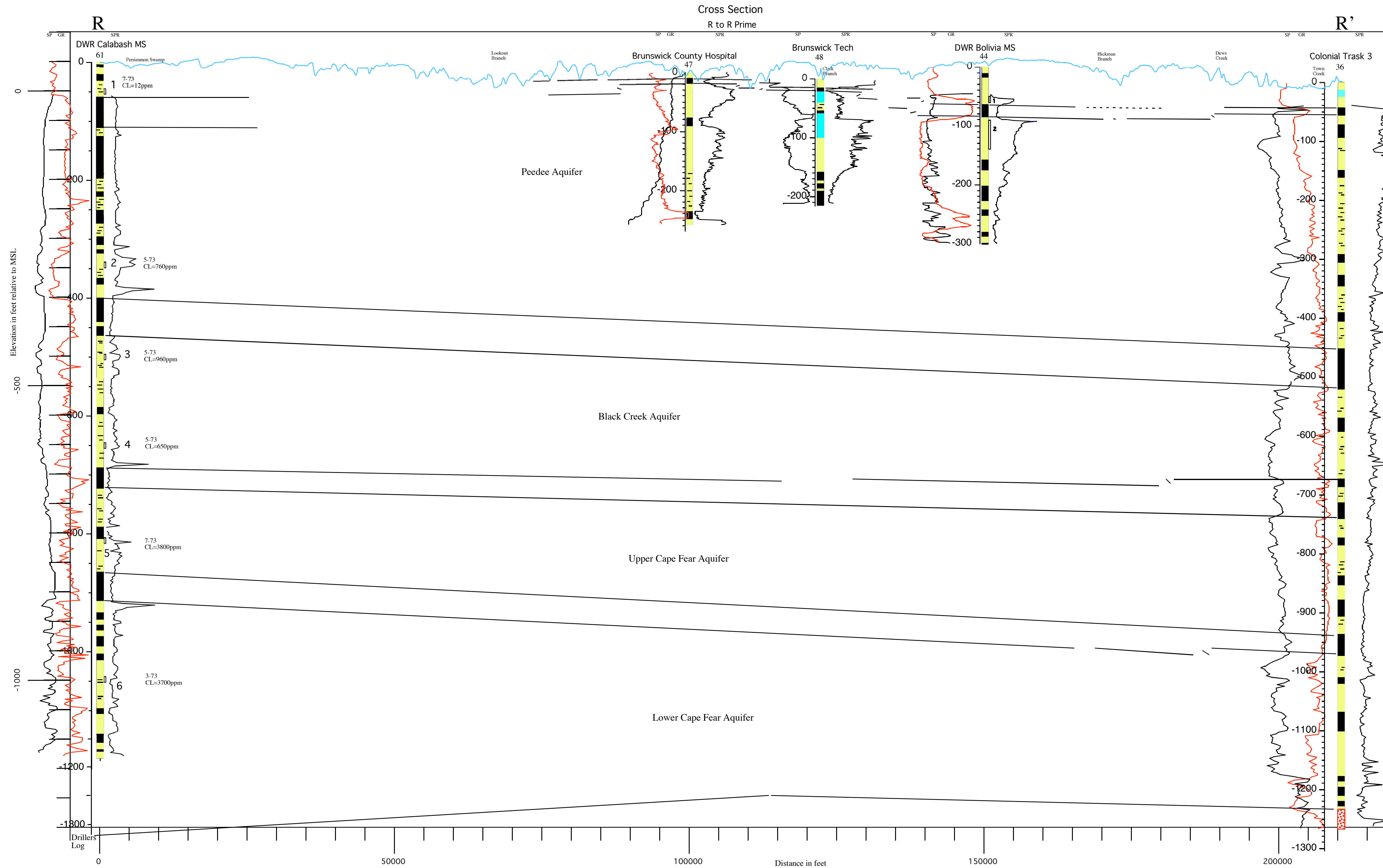
Plate 19. Southwest to Northeast Hydrogeologic Cross Section R-R' through Brunswick County, NC
