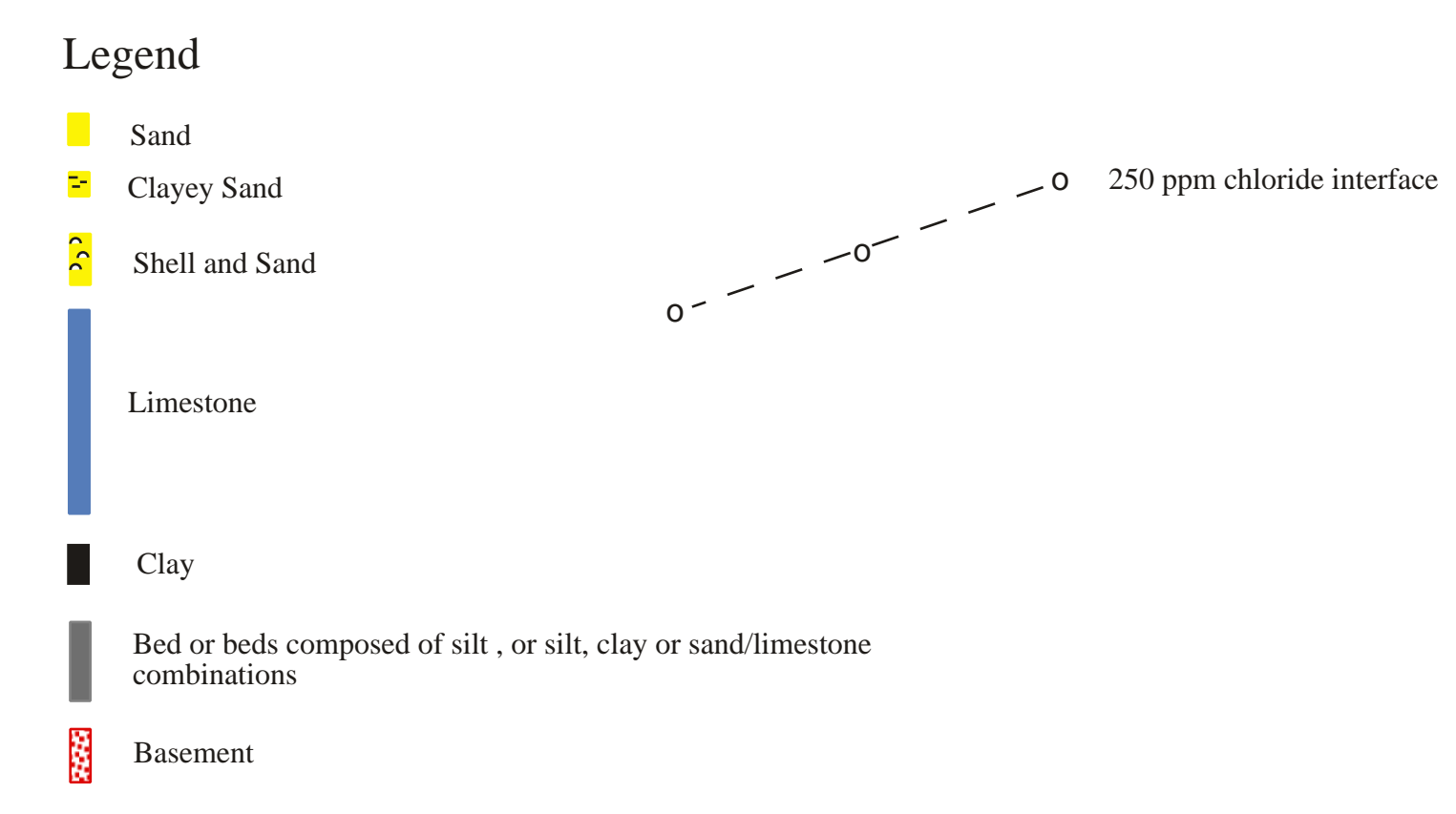
Plate 22. Northwest to Southeast Hydrogeologic Cross Section U-U' through Sampson, Duplin, and Pender Counties, NC
