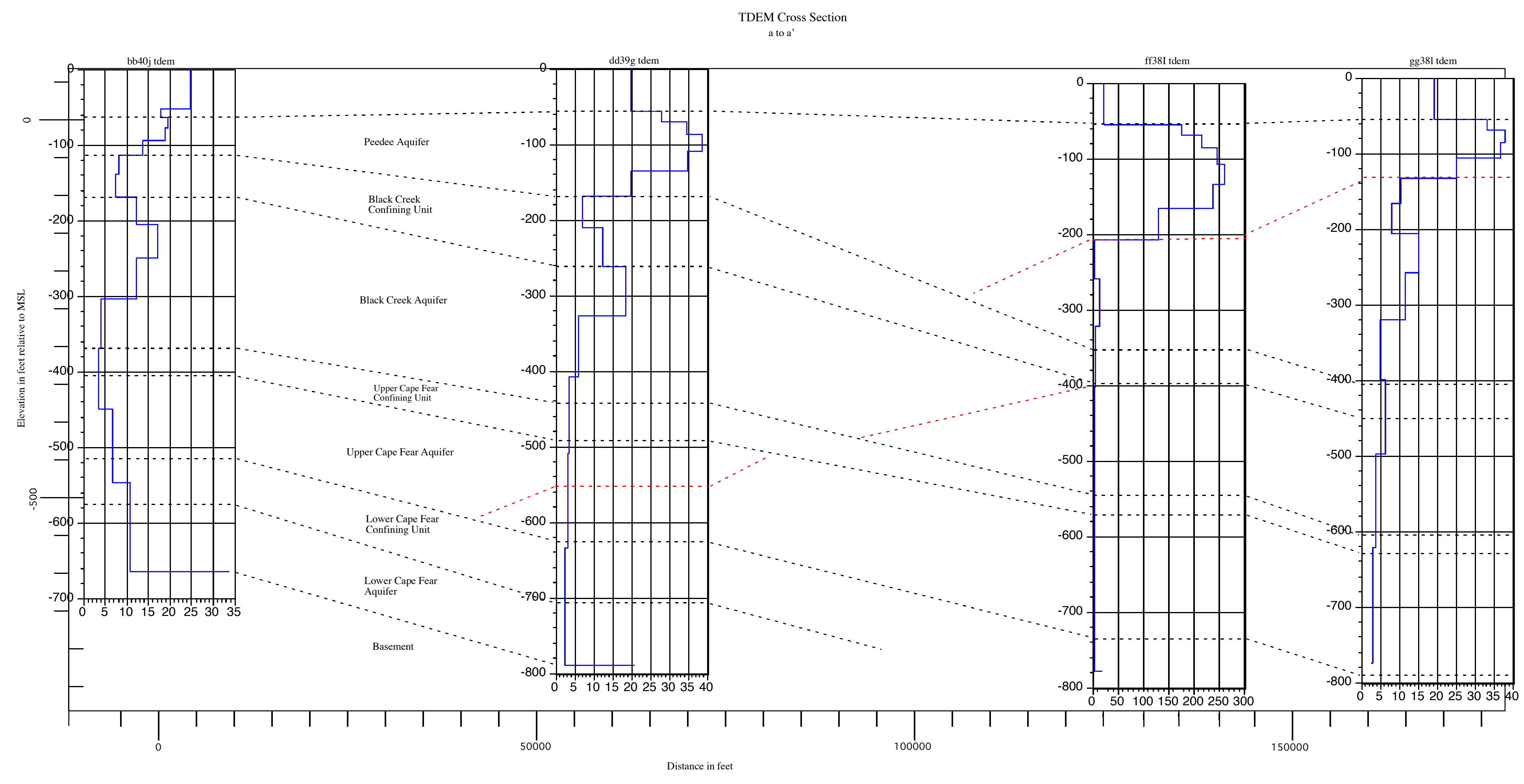
Plate 24. Time Domain Electromagnetic Resistivity Profile a-a' through Columbus and Brunswick Counties, NC
